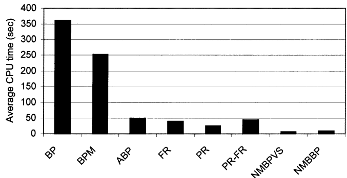
Fig. 5. Numeric font learning problem: Average CPU time for convergence of each training algorithm.
