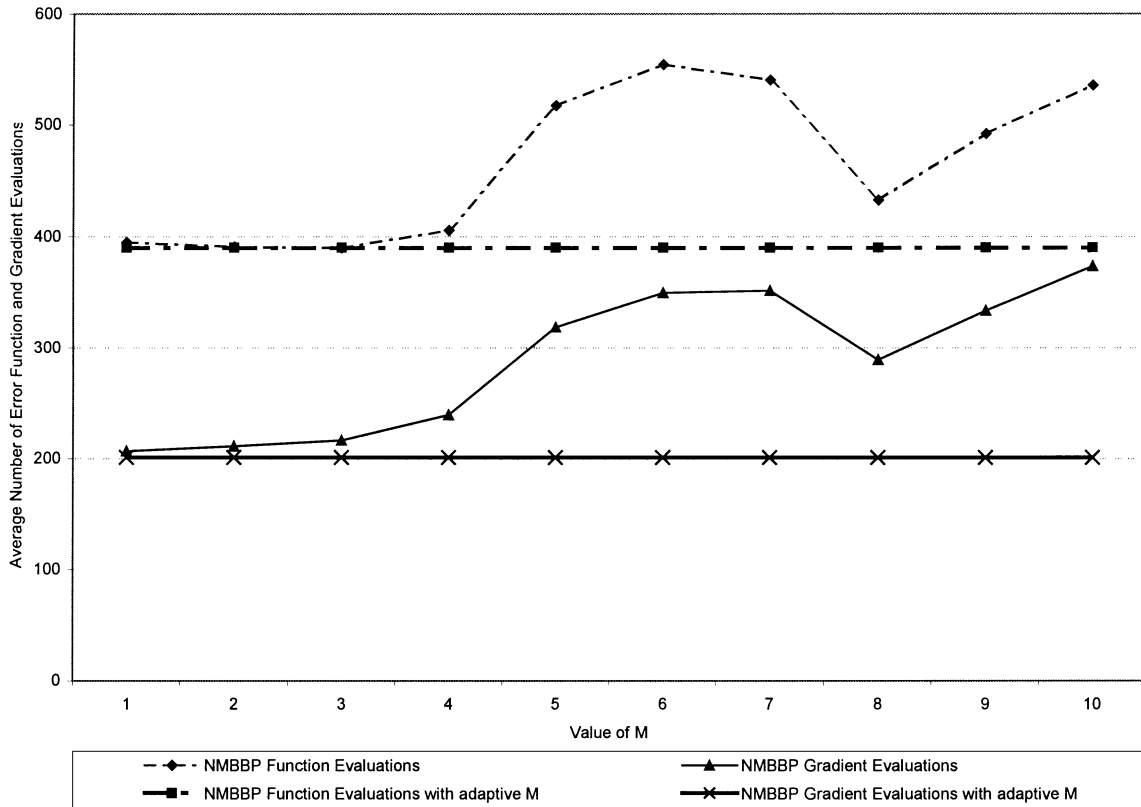
Fig. 8. Texture classification problem: Average number of error function and gradient evaluations for the NMBBP method with respect to different values of M .
