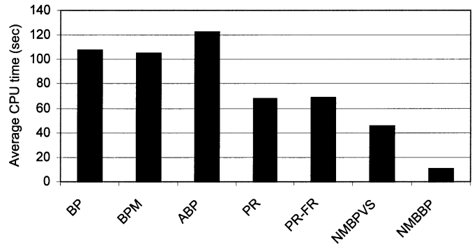
Fig. 4. Alphabetic font learning problem: Average CPU time for convergence of each training algorithm.
