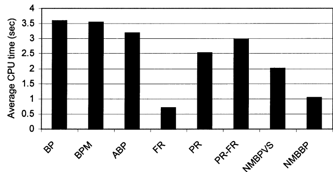
Fig. 3. Function approximation problem: Average CPU time for convergence of each training algorithm.
